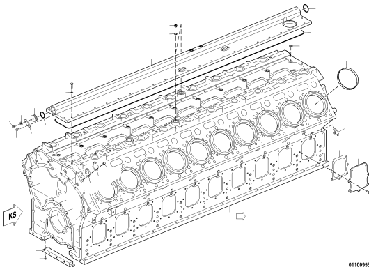
CRANKCASE X00030265
