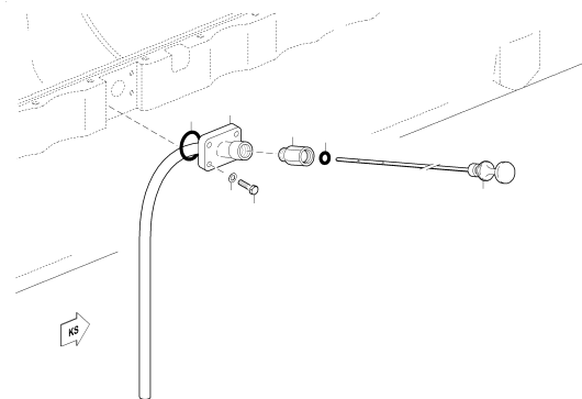
OIL FILLER NECK FOR DEEP OIL PAN XS596010.00043
